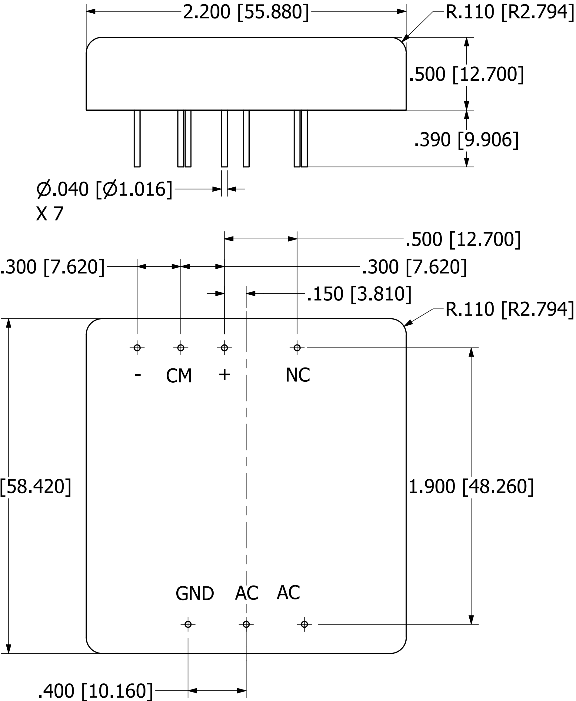
BOTTOM VIEW
